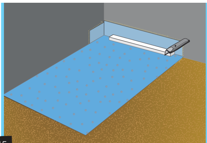
15 Bond waterproof membrane to the shower area with C2 flexible cement based adhesive and lap up the walls.
