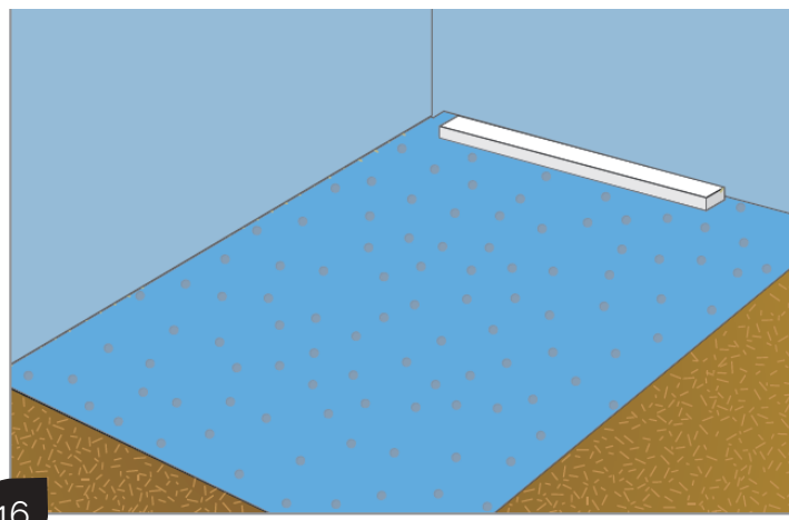
16 The walls can also be waterproofed with the membrane if desired. Then install the wall tiles.
